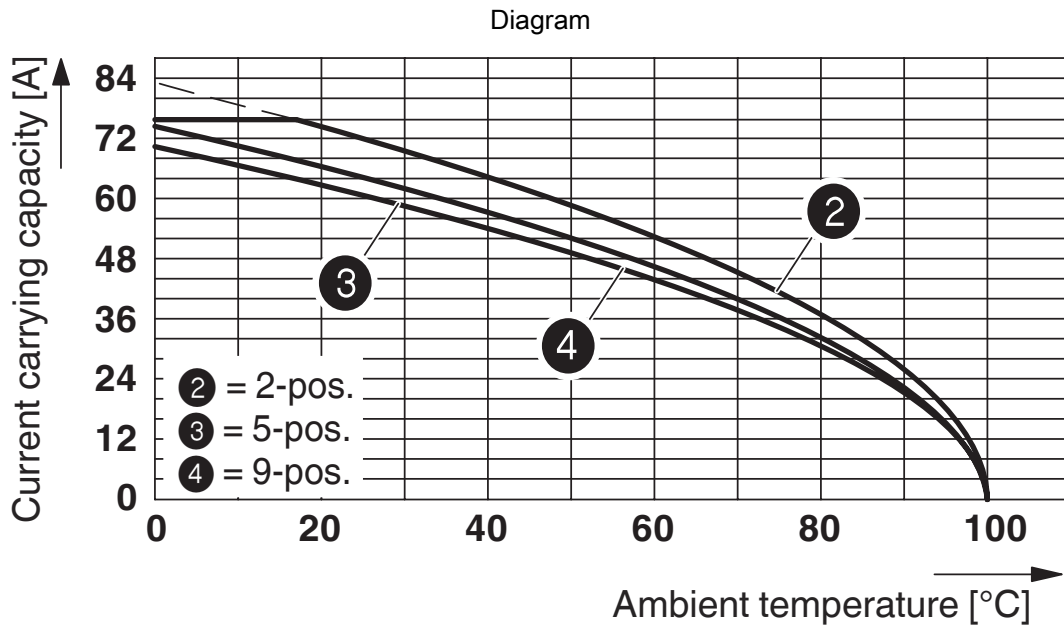
Derating curve for: IPC 16/...-ST-10,16 with IPC 16/...-G-10,16
