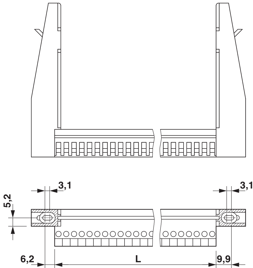
Dimensional drawing
