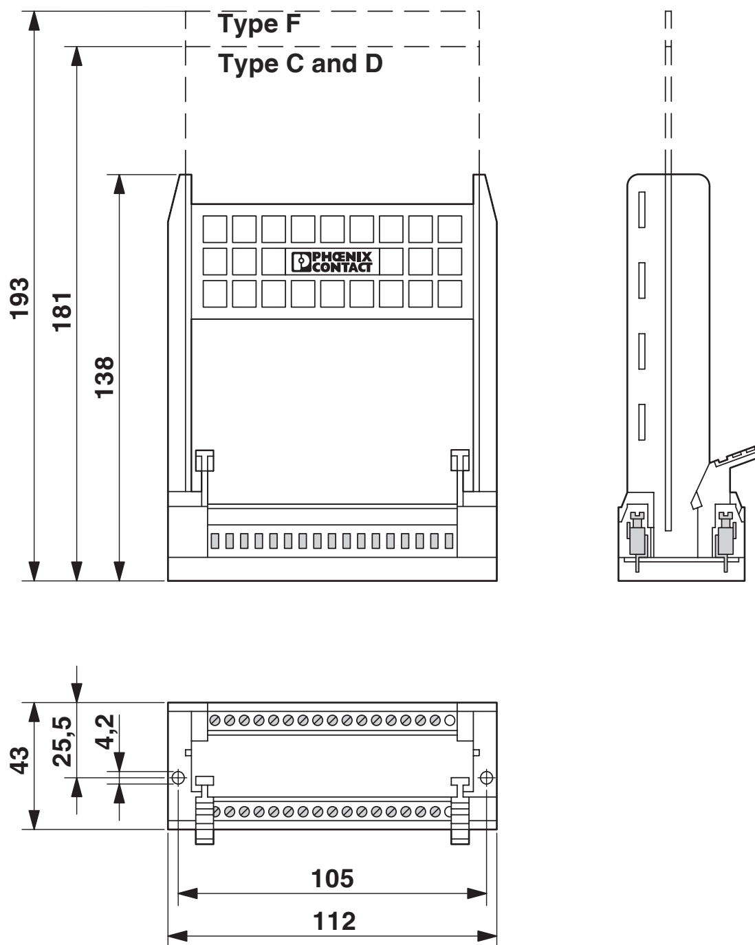
Dimensional drawing
