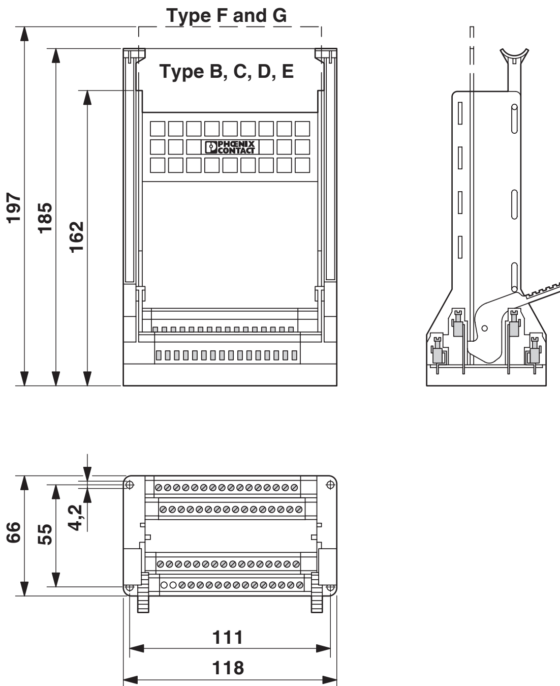
Dimensional drawing
