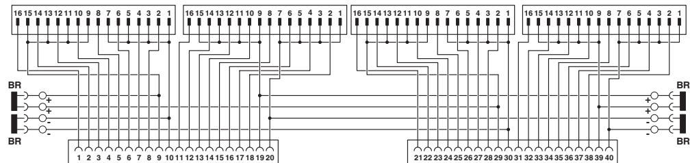
Circuit diagram
