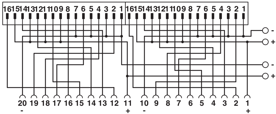
Circuit diagram
