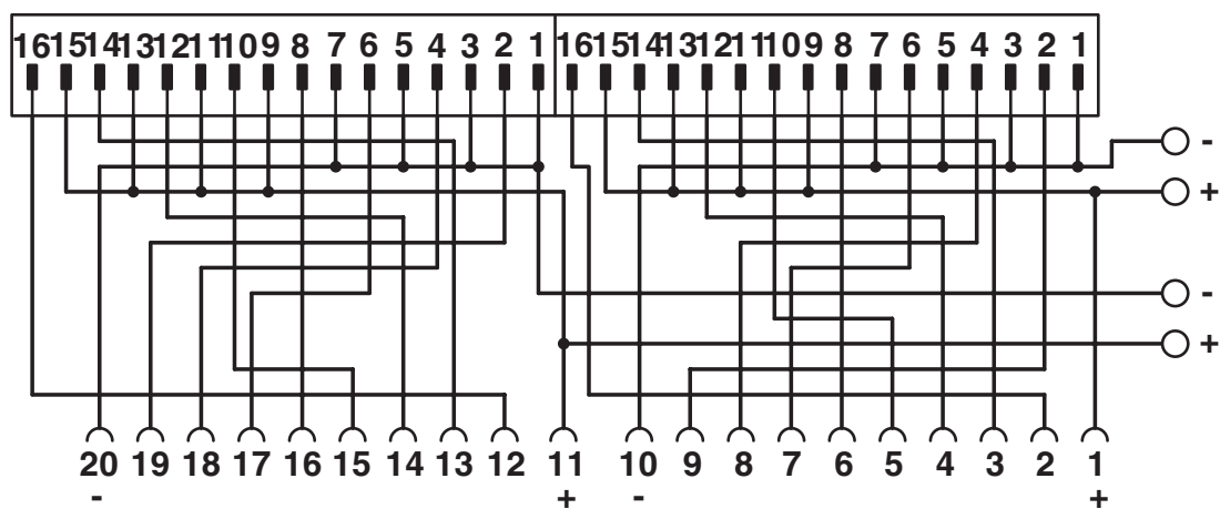
Circuit diagram
