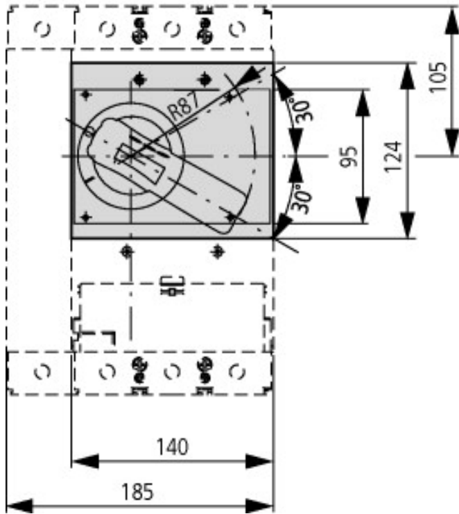
Rotary drive
