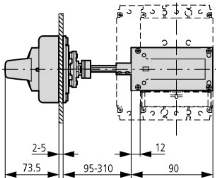
NZM1-XS(R)-L
