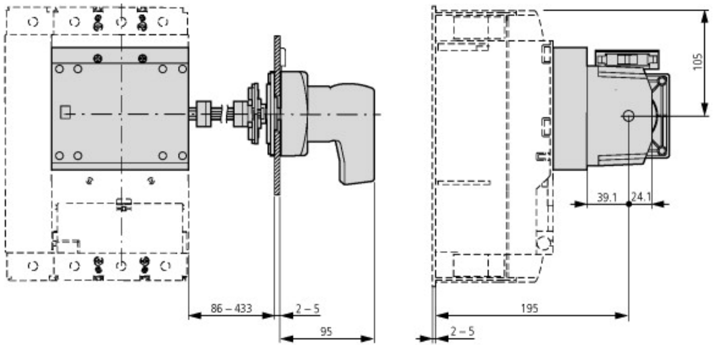
NZM3-XS(R)-L
