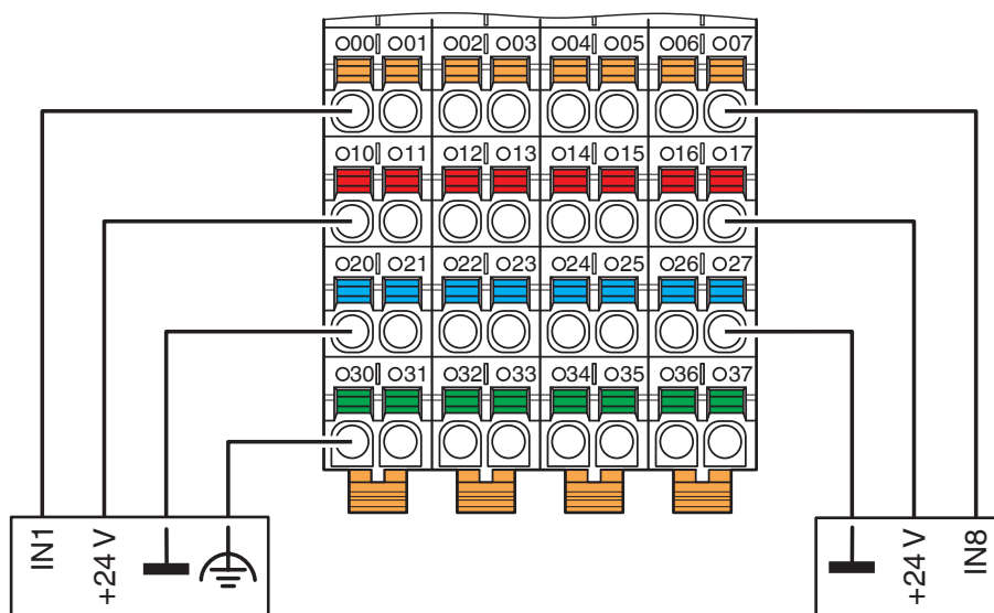
Connection diagram
