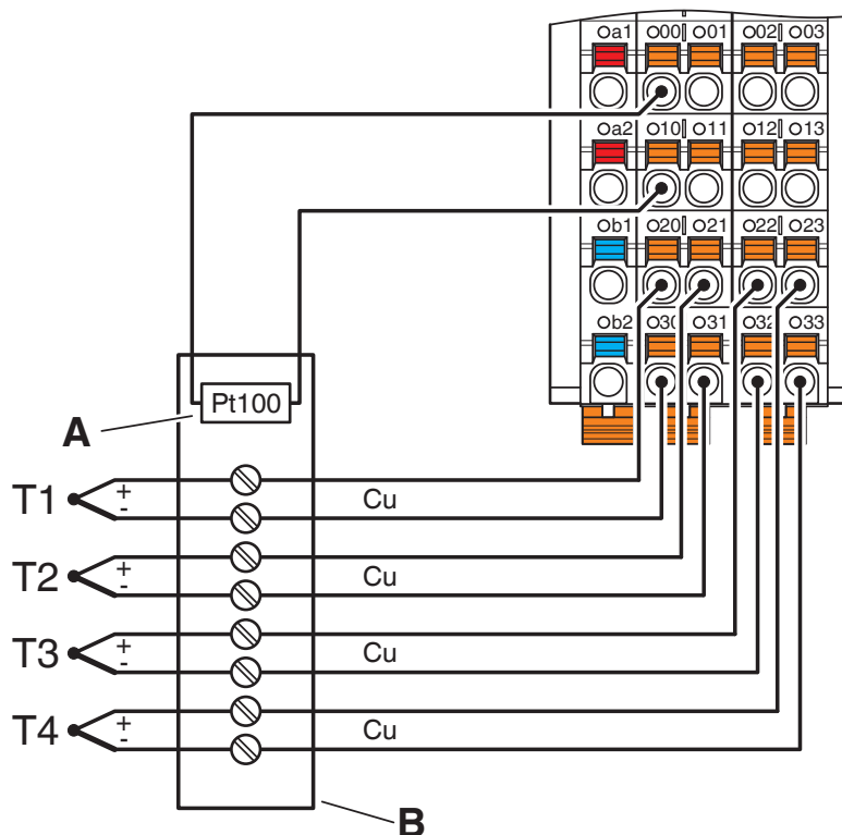
Connection diagram
