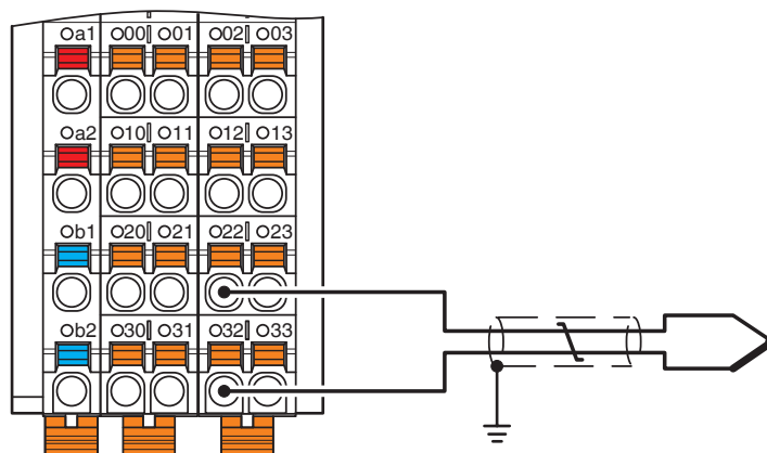
Connection diagram
