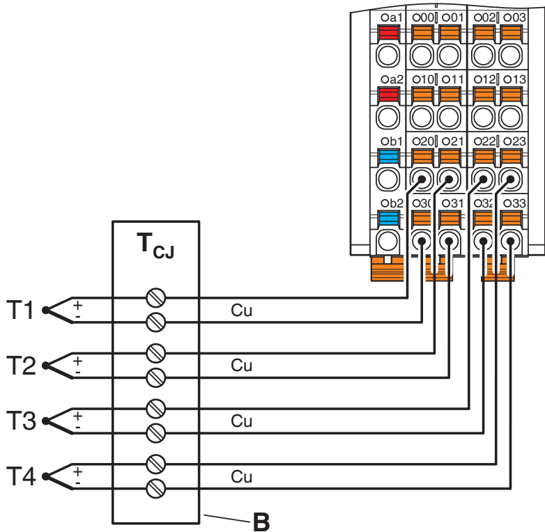
Connection diagram
