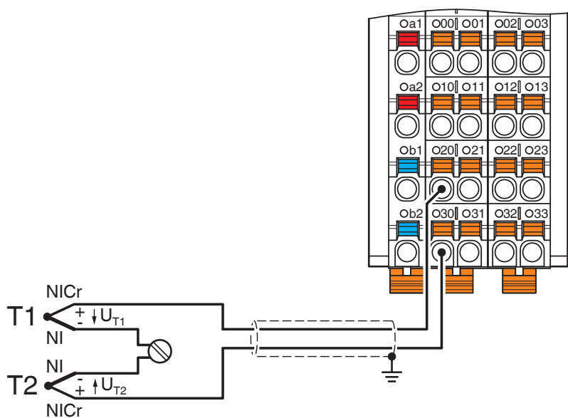
Connection diagram
