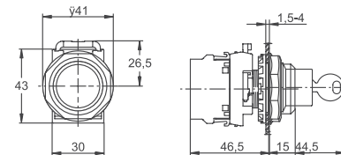
Key-operated selector switch
