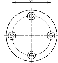
Drilling Plan for Signal Towers K 70
