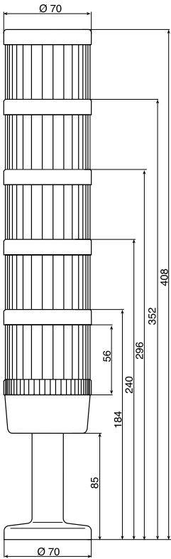
Signal Towers K 70
