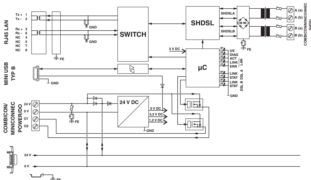
Circuit diagram
