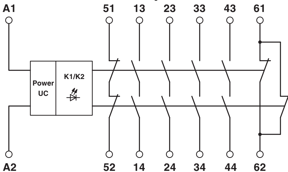
Block diagram
