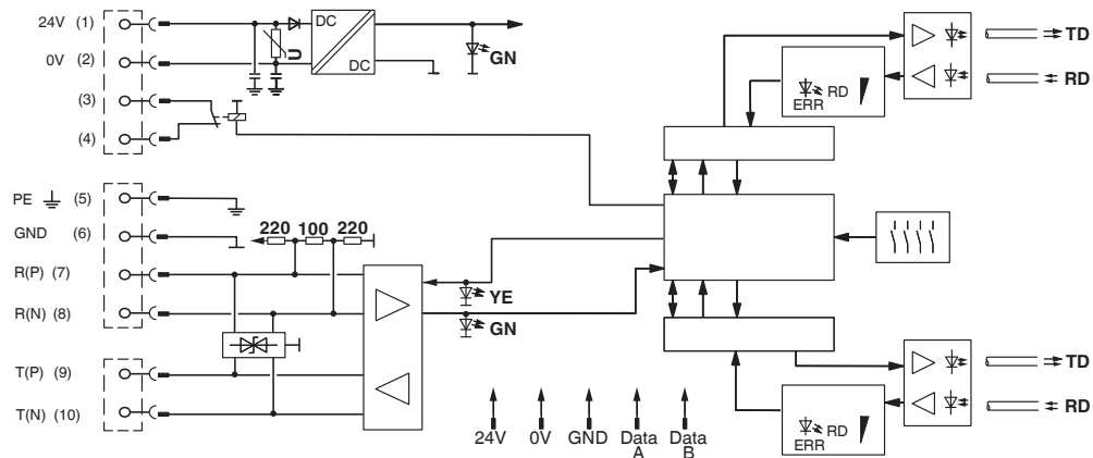
Block diagram
