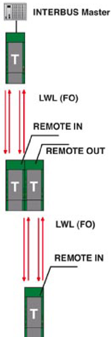
Application drawing
