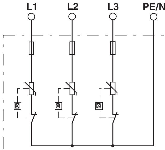
Circuit diagram
