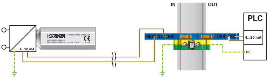
Application drawing
