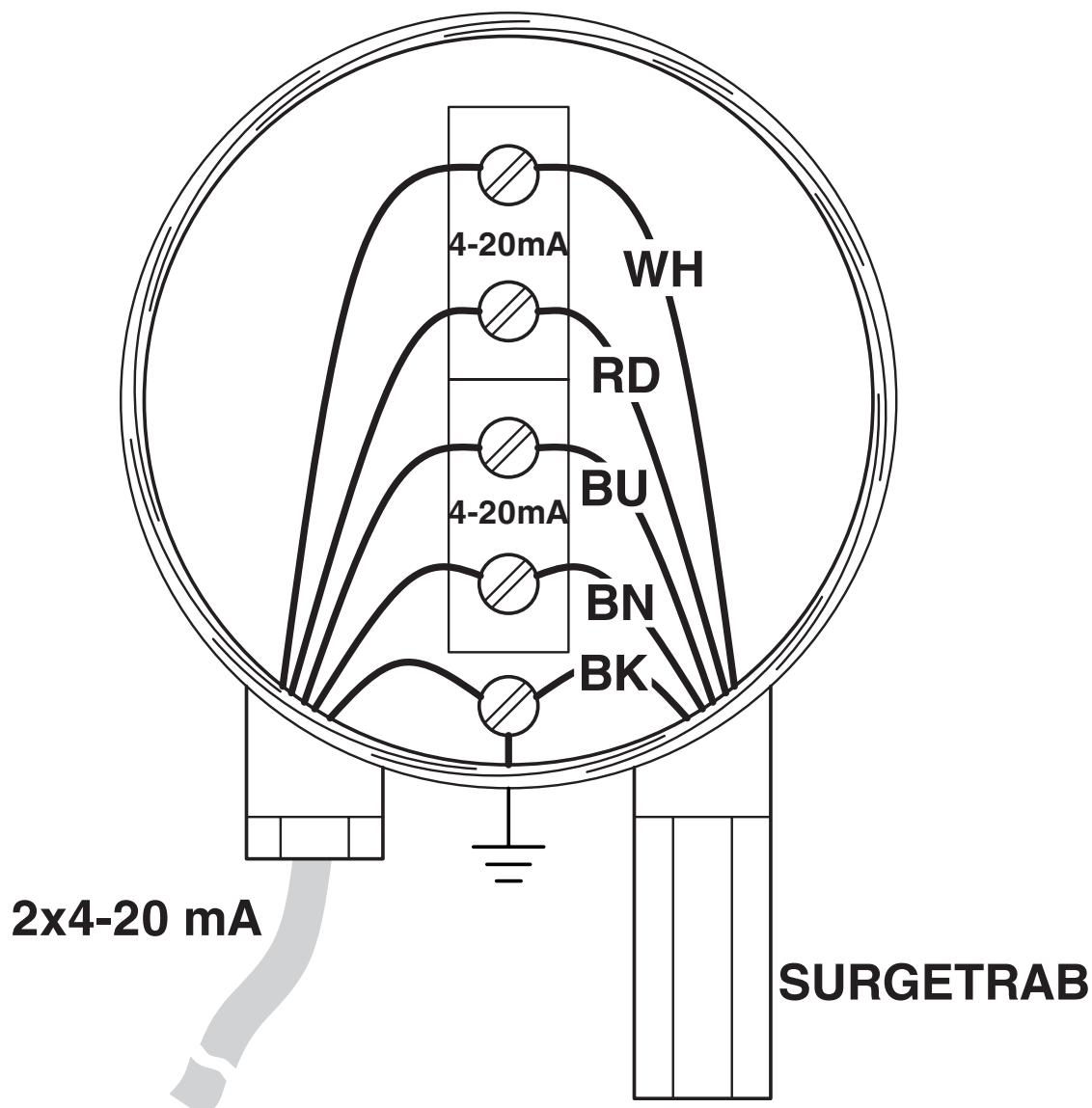
Application drawing
