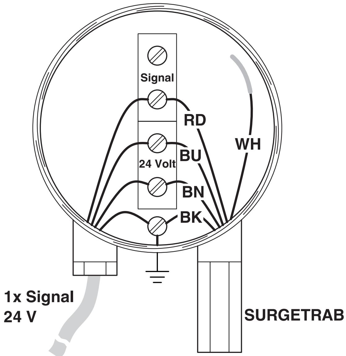
Application drawing
