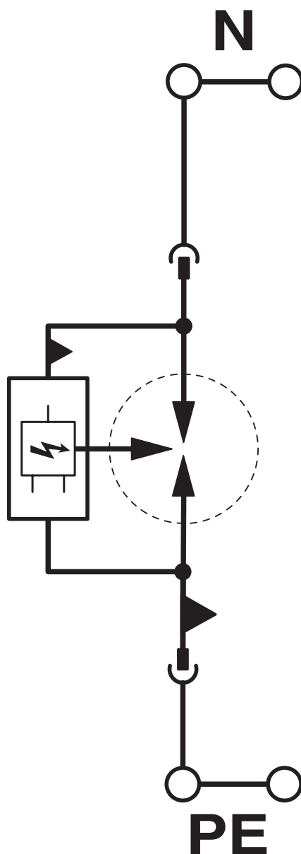
Circuit diagram
