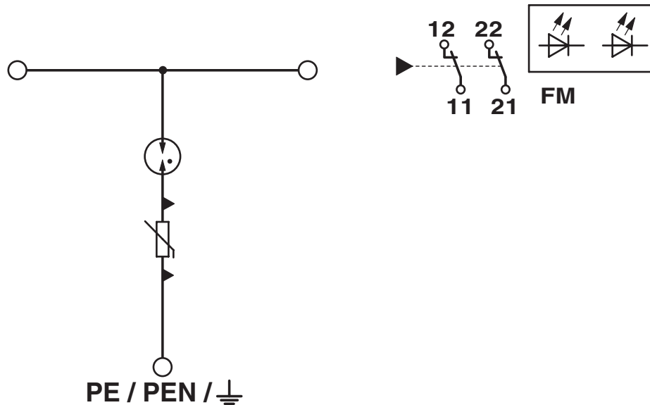
Circuit diagram
