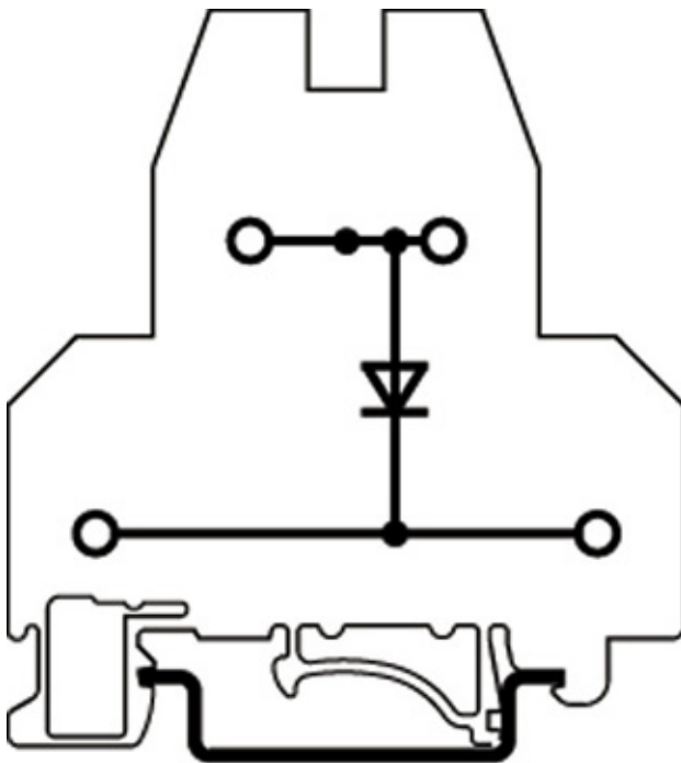
Circuit diagram
