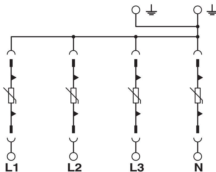
Circuit diagram
