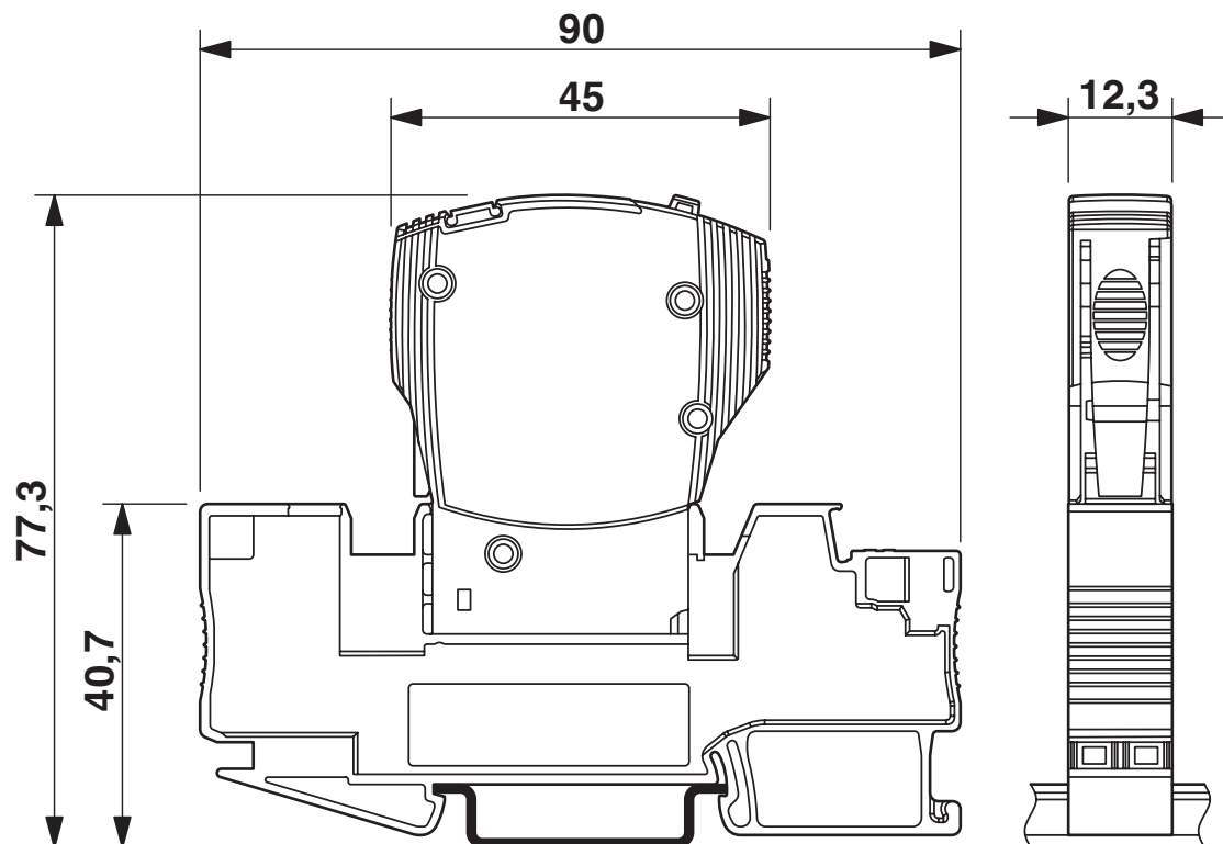
Dimensional drawing
