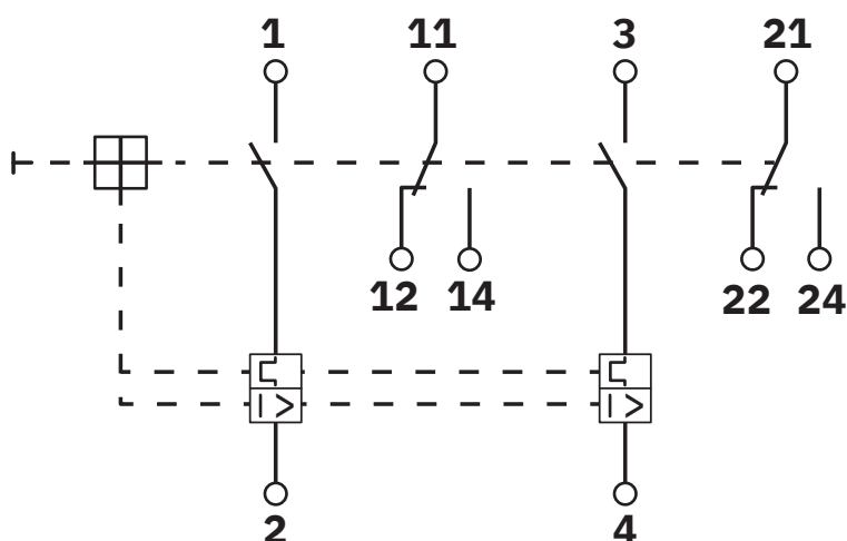
Circuit diagram
