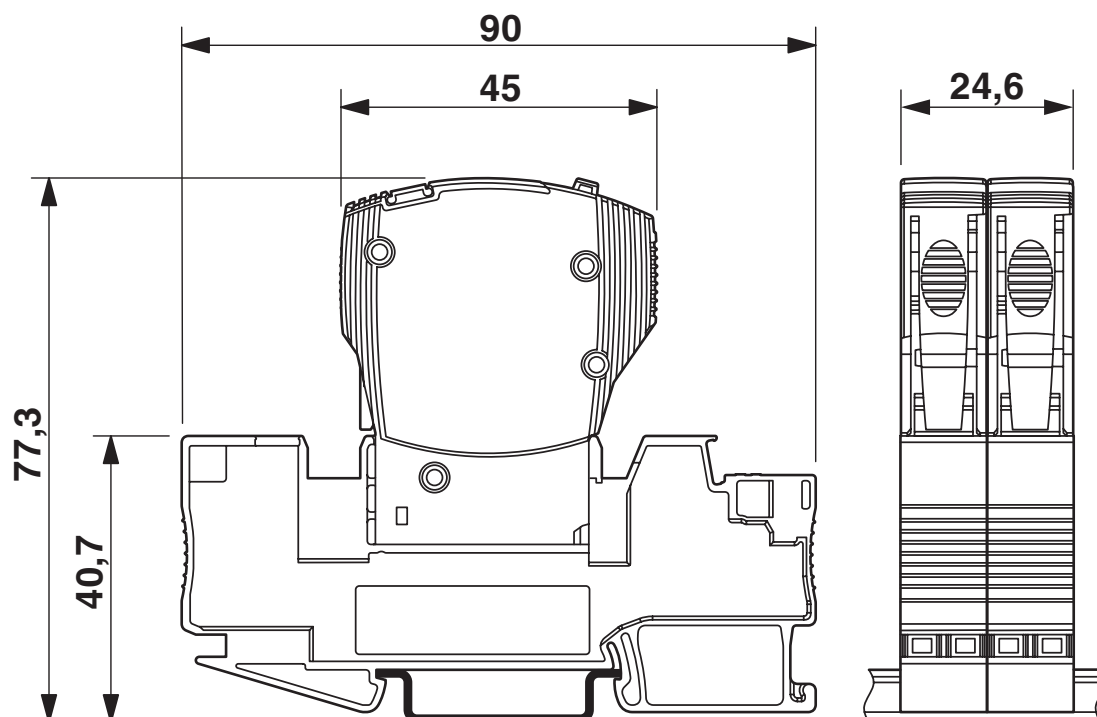
Dimensional drawing
