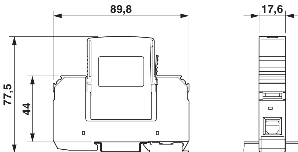
Dimensional drawing
