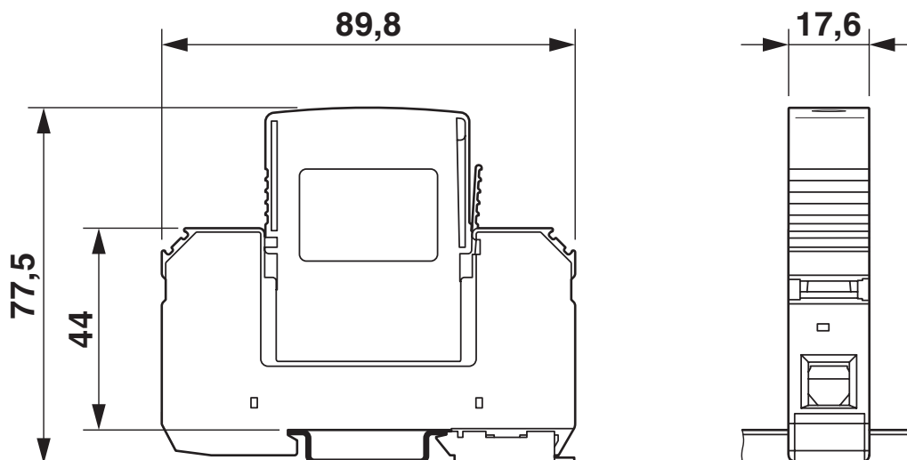
Dimensional drawing
