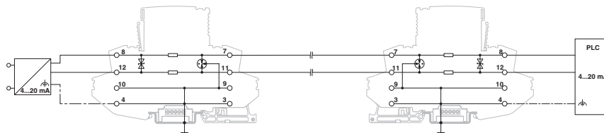
Application drawing
