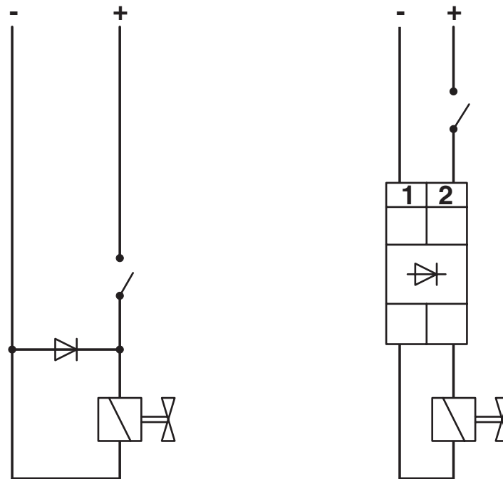
Circuit diagram
