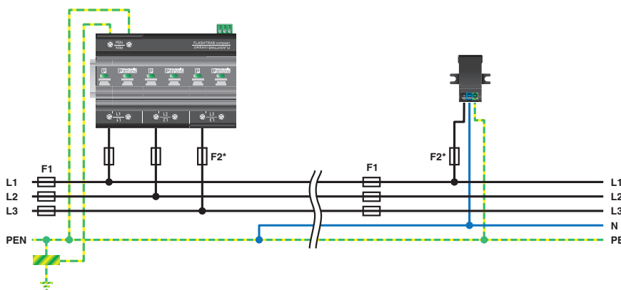
Application drawing
