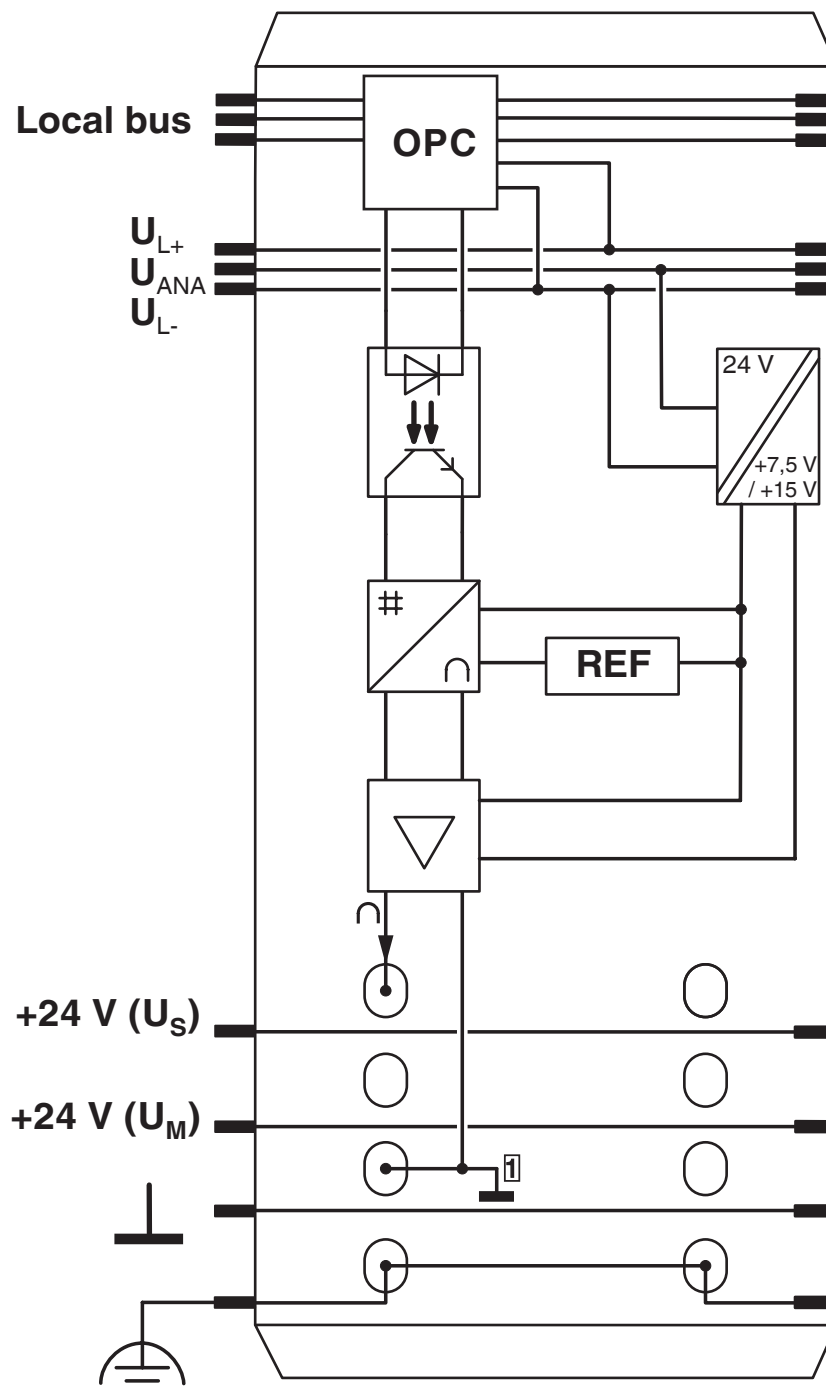
Block diagram
