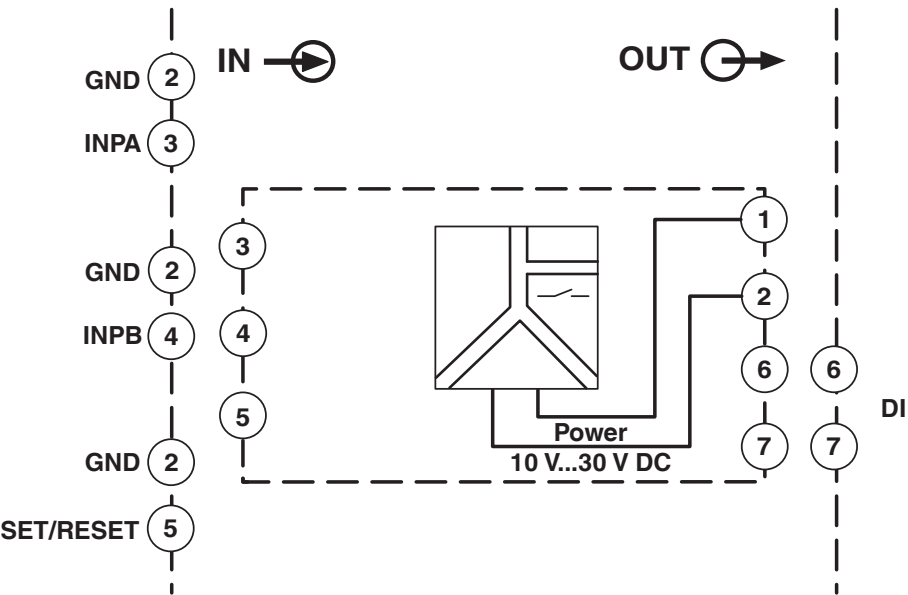
Block diagram
