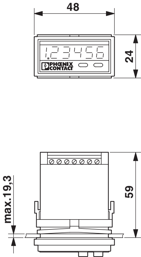
Dimensional drawing
