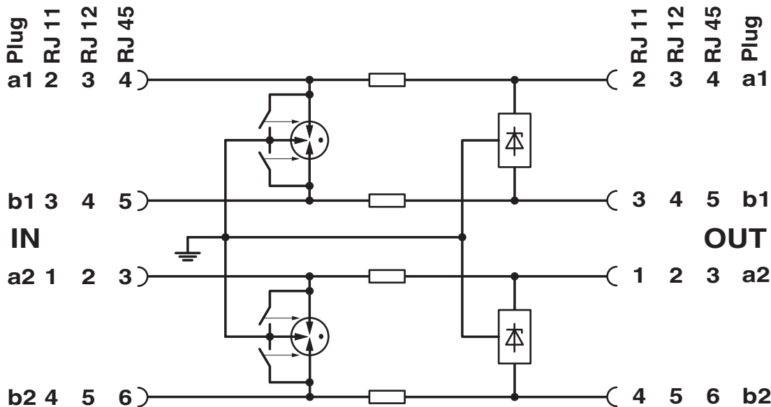
Circuit diagram
