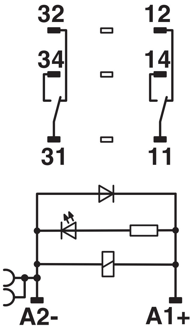
Circuit diagram
