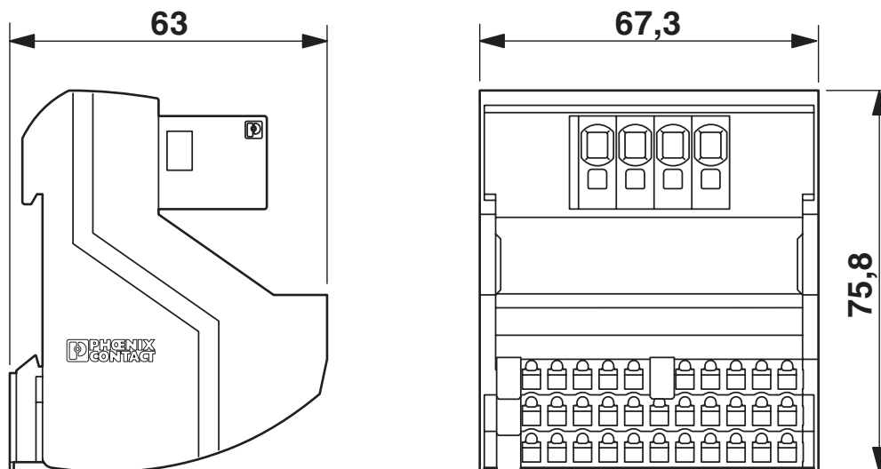
Dimensional drawing
