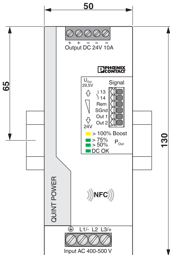
Dimensional drawing
