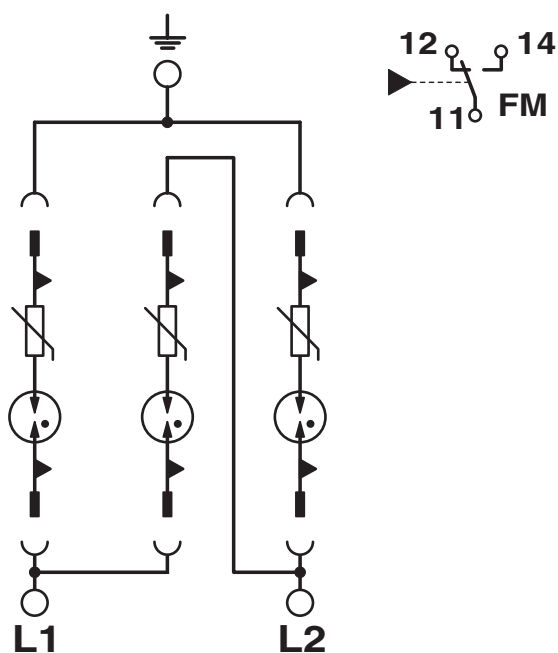
Circuit diagram
