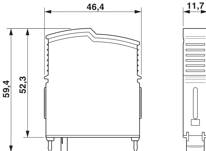
Dimensional drawing
