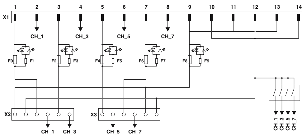
Circuit diagram
