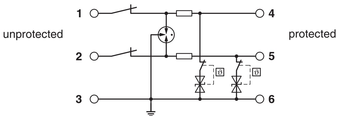
Circuit diagram
