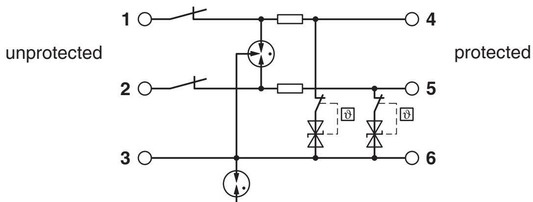
Circuit diagram
