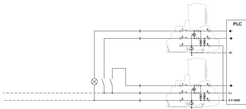
Application drawing
