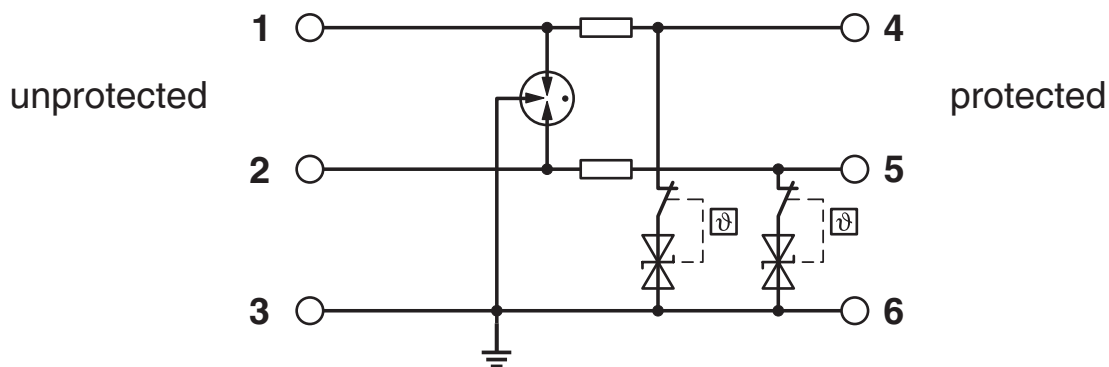
Circuit diagram
