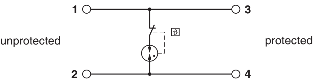
Circuit diagram
