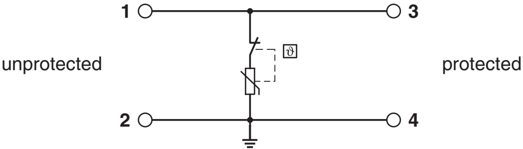
Circuit diagram
