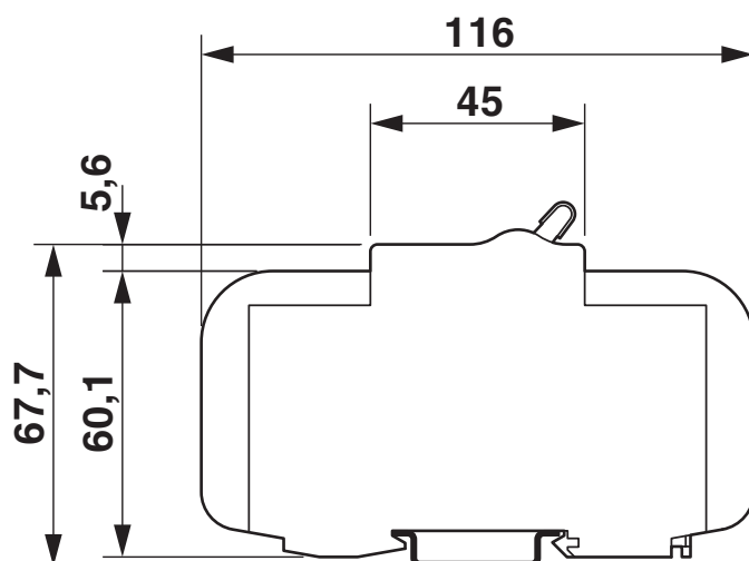
Dimensional drawing
