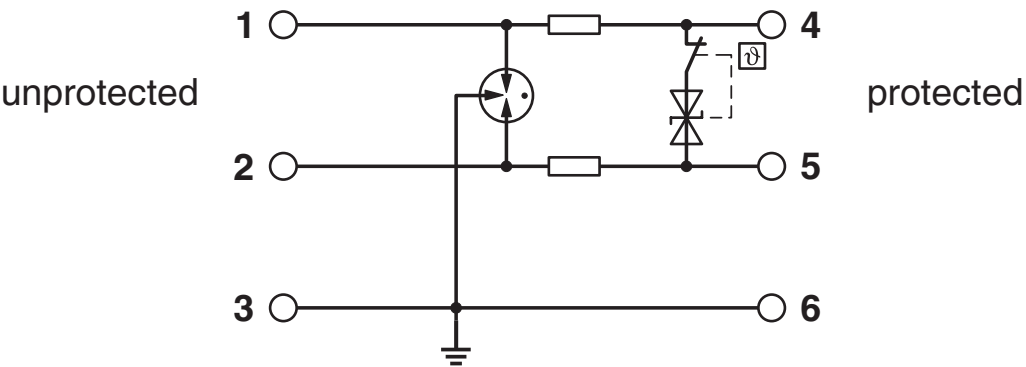
Circuit diagram
