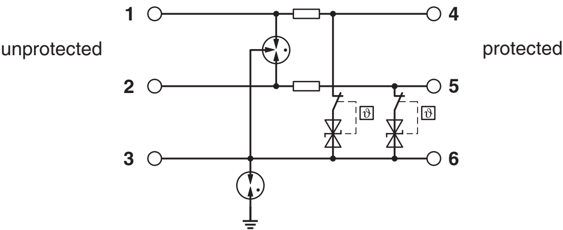
Circuit diagram
