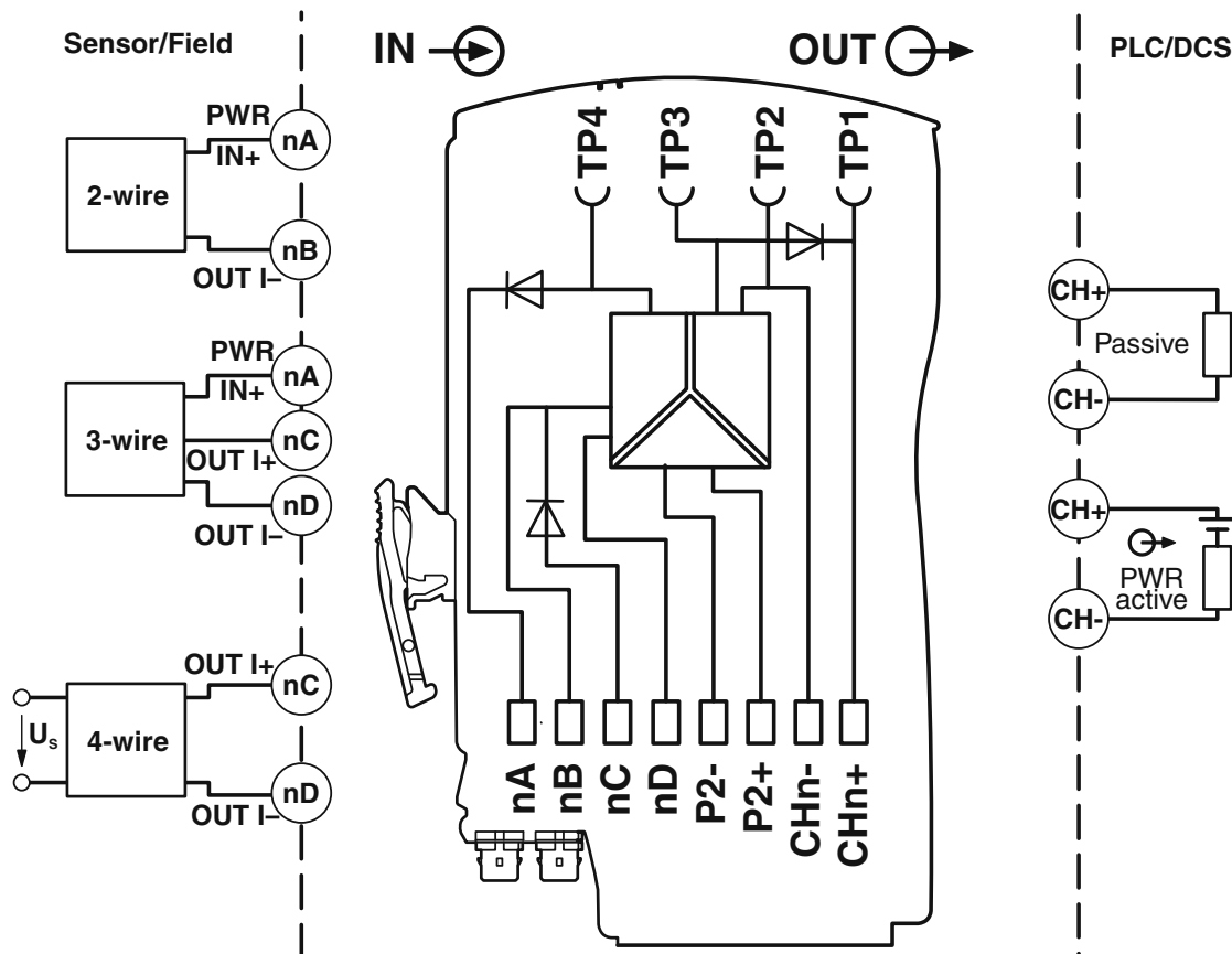
Block diagram
